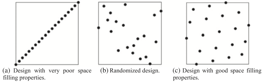
Exemples of Latin hypercube designs with d = 2 dimensions and p = 20 points
